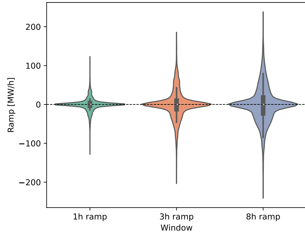
Heat Bus Ramping Distribution
