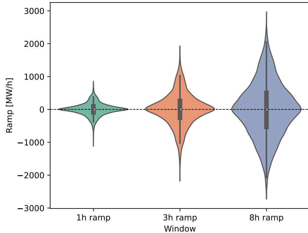
Electricity Bus Ramping Distribution
