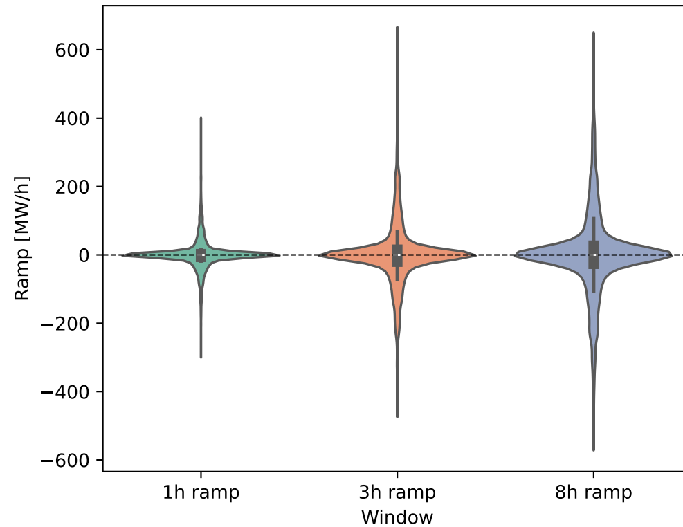
Hydrogen Bus Ramping Distribution
